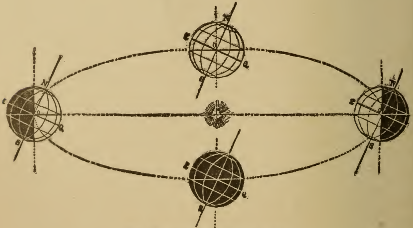
Fig. 172. ORBIT OF THE EARTH.
